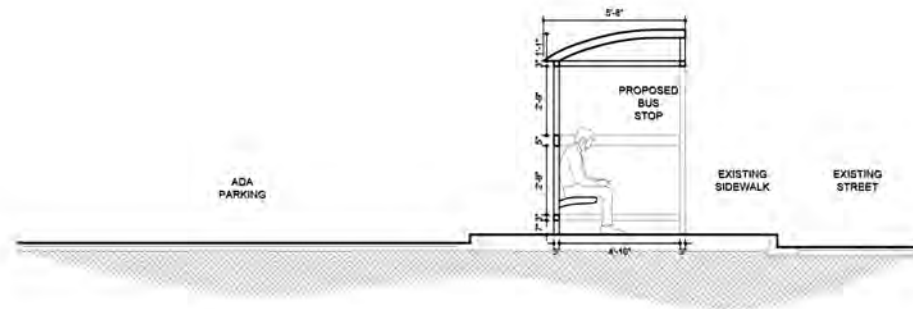
PROPOSED TROLLEY STOP SECTION
