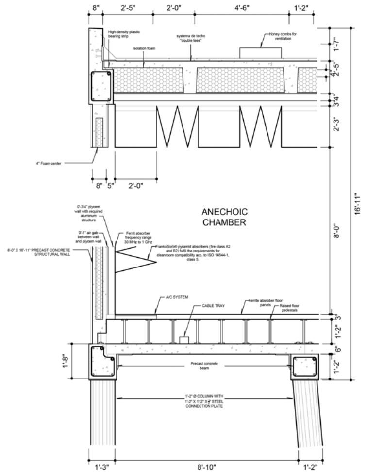
ANECHOIC CHAMBER WALL SECTION
