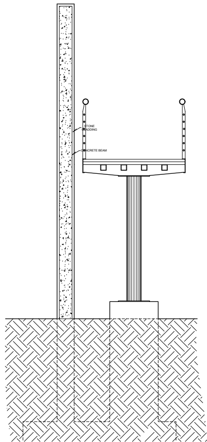
TYP. CONCRETE WALL & BRIDGE SECTION
