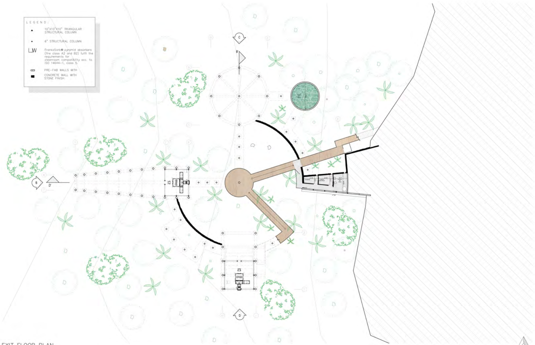
EXIT FLOOR PLAN
