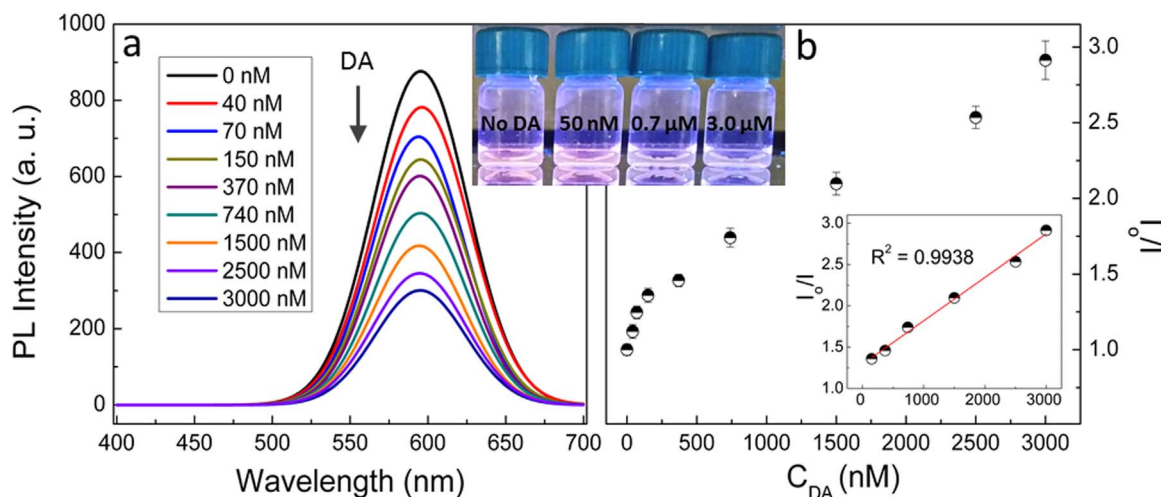
Fig. 3. Phosphorescence emission spectra (a) of L-cys capped ZnS:Mn QDs in the presence of different concentrations of DA (0–3000 nM). Stern-Volmer plots of I_0/I as a function of the DA concentration (0–3000 nM) (b). Lower inset shows the expanded linear region of the calibration curve. Upper inset shows the optical images of the phosphorescence quenching that undergoes the QDs as DA concentration increases (excitation light: 302 nm).
